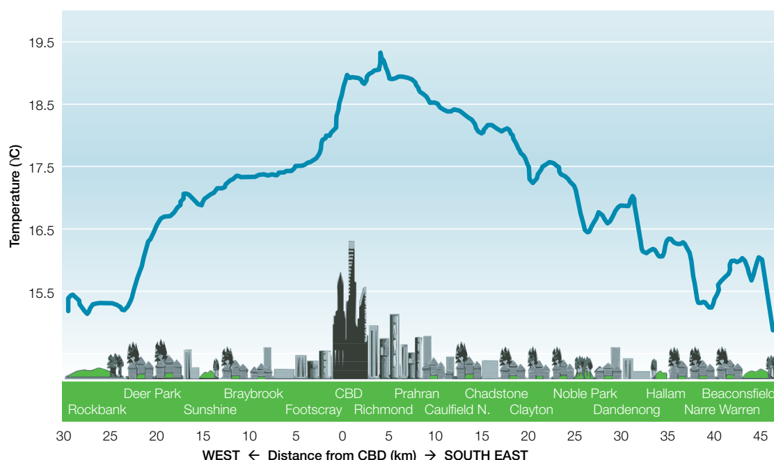
Figure 2: Spatial variability of the Melbourne urban heat island (1 am, 23 March 2006)
